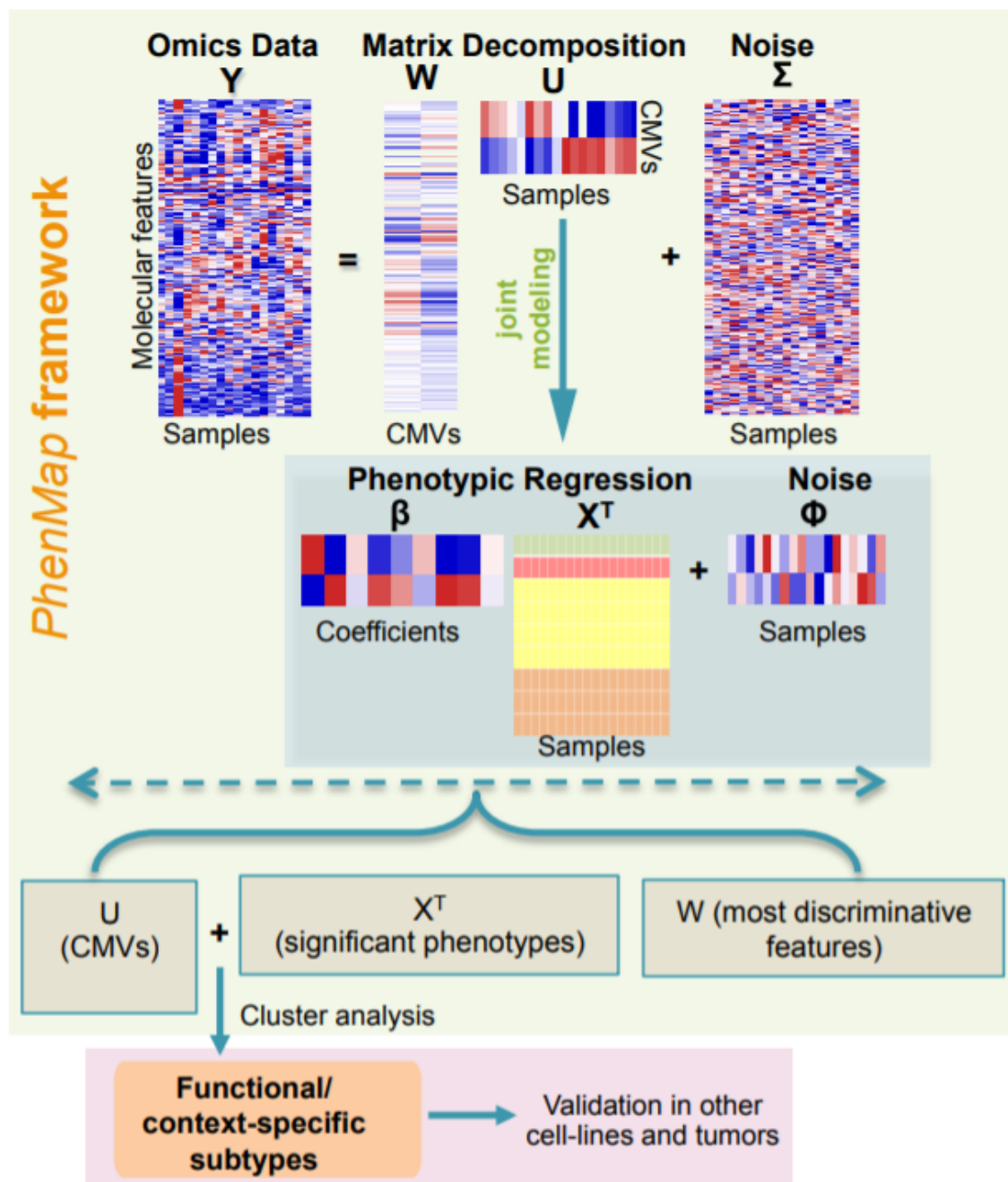
Figure 1. A flowchart of the steps involved in PhenMap framework. PhenMap is a machine-learning approach that maps the high-dimensional omics data matrix Y (with features or genes on the rows) to a low-dimensional matrix of context-specific mapping variables (CMVs), U (with samples on the columns) using a projection (loadings) matrix W (features on the rows). Matrix \Sigma (noise) represents
